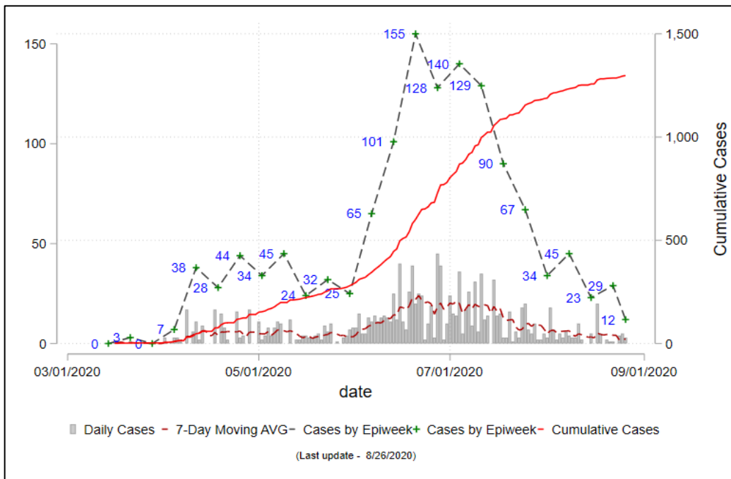
Figure 2: Epi-curve for COVID 19 Cases in Liberia, 14 March – 26 August 2020
