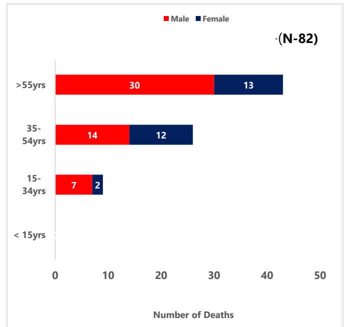
Figure 6: Distribution of Confirmed COVID-19 Deaths by Age and Sex, Liberia, March 16- August 26, 2020
