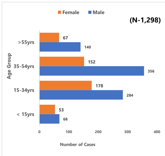
Figure 5: Distribution of Confirmed COVID-19 Cases by Age and Sex, Liberia, March 16- August 26, 2020
